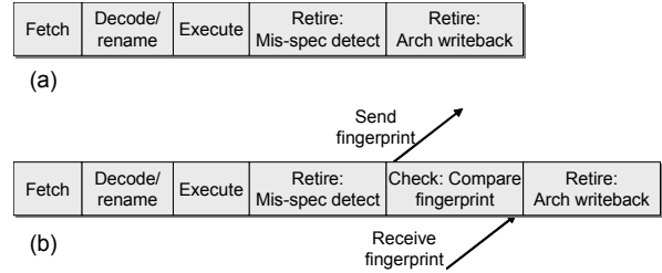
Figure 3. (a) Baseline pipeline and (b) a pipeline with fingerprint checks before retirement.
