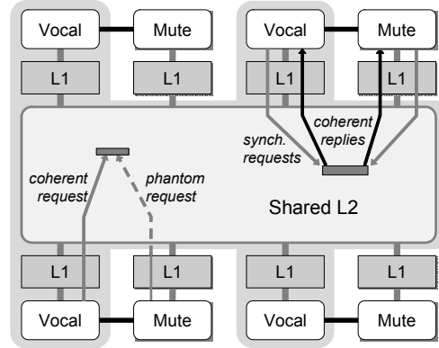
Figure 2. The Reunion architecture.
